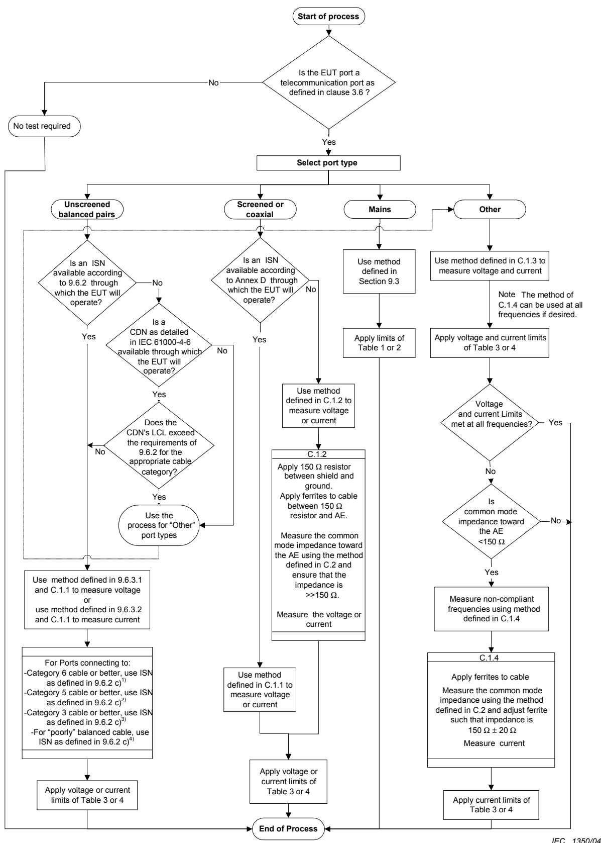
Figure C.6 – Flowchart for selecting test method
