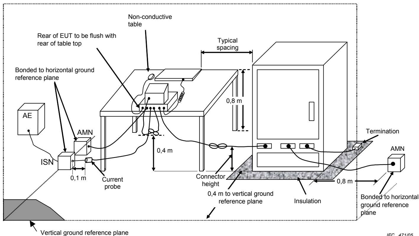
Figure 9 – Example test arrangement for combinations of equipment (conducted emission measurement)
